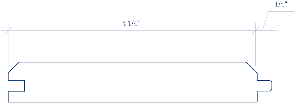
IL 915 Shown as 11/16 x 4 1/2 (Available in all thicknesses and widths)
