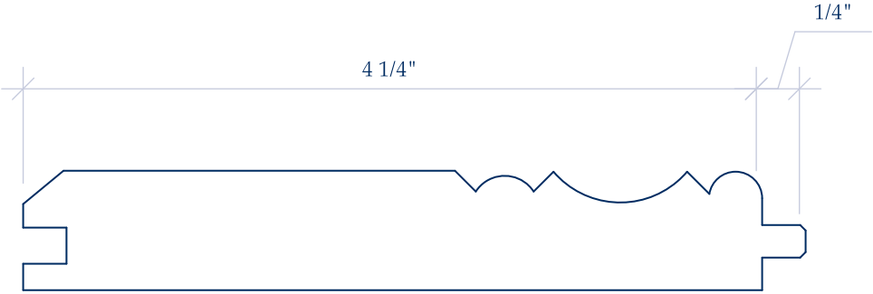
IL 917 Shown as 11/16 x 4 1/2 (Available in all thickness and widths)
